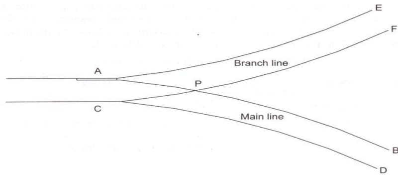
(Fig: Negative superelevation)
