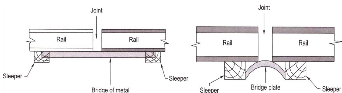
(Bridge joint with metal flat Joint)
